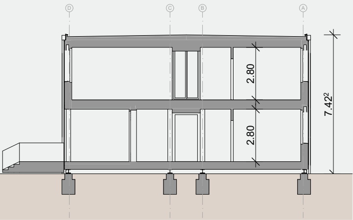
Section transversale
